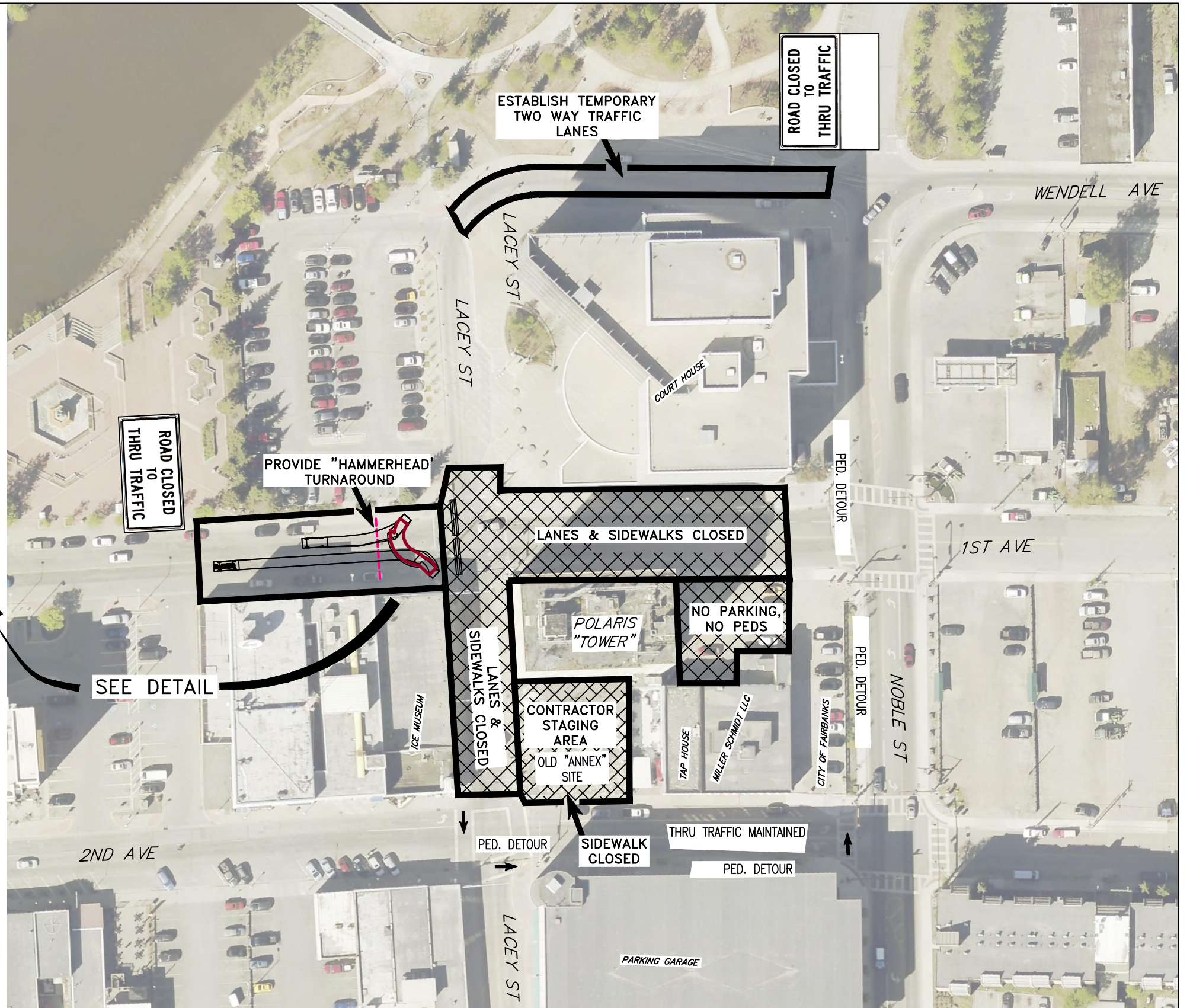
EXHIBIT B Phase 2: Tower Demolition Vehicle Traffic Routes & Closures
