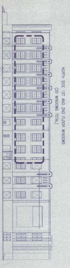
4 WORK AREAS NORTH ELEVATION G2 1/16" = 1'-0"
