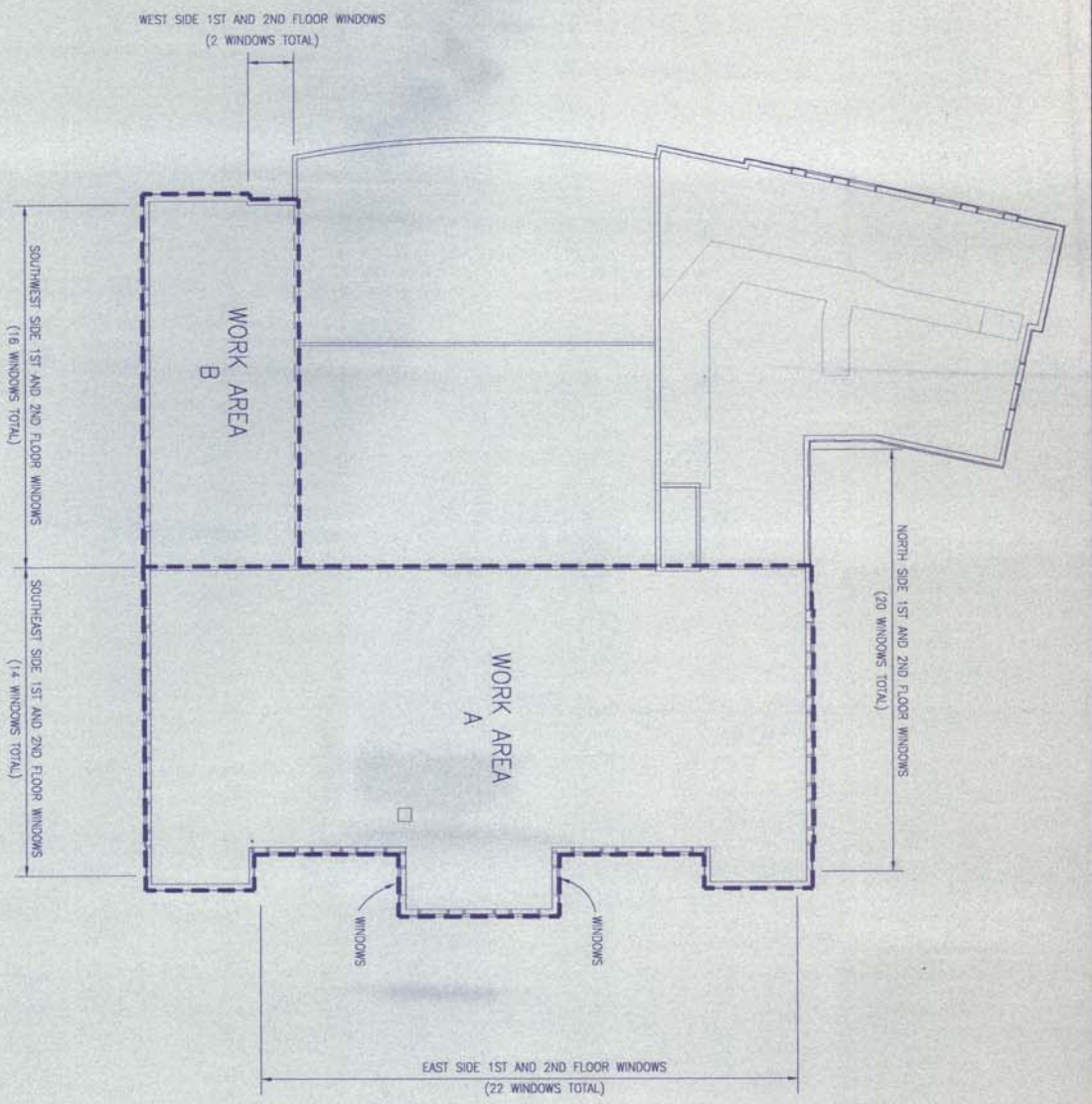
1 WORK AREAS PLAN G2 1/16" = 1'-0"
