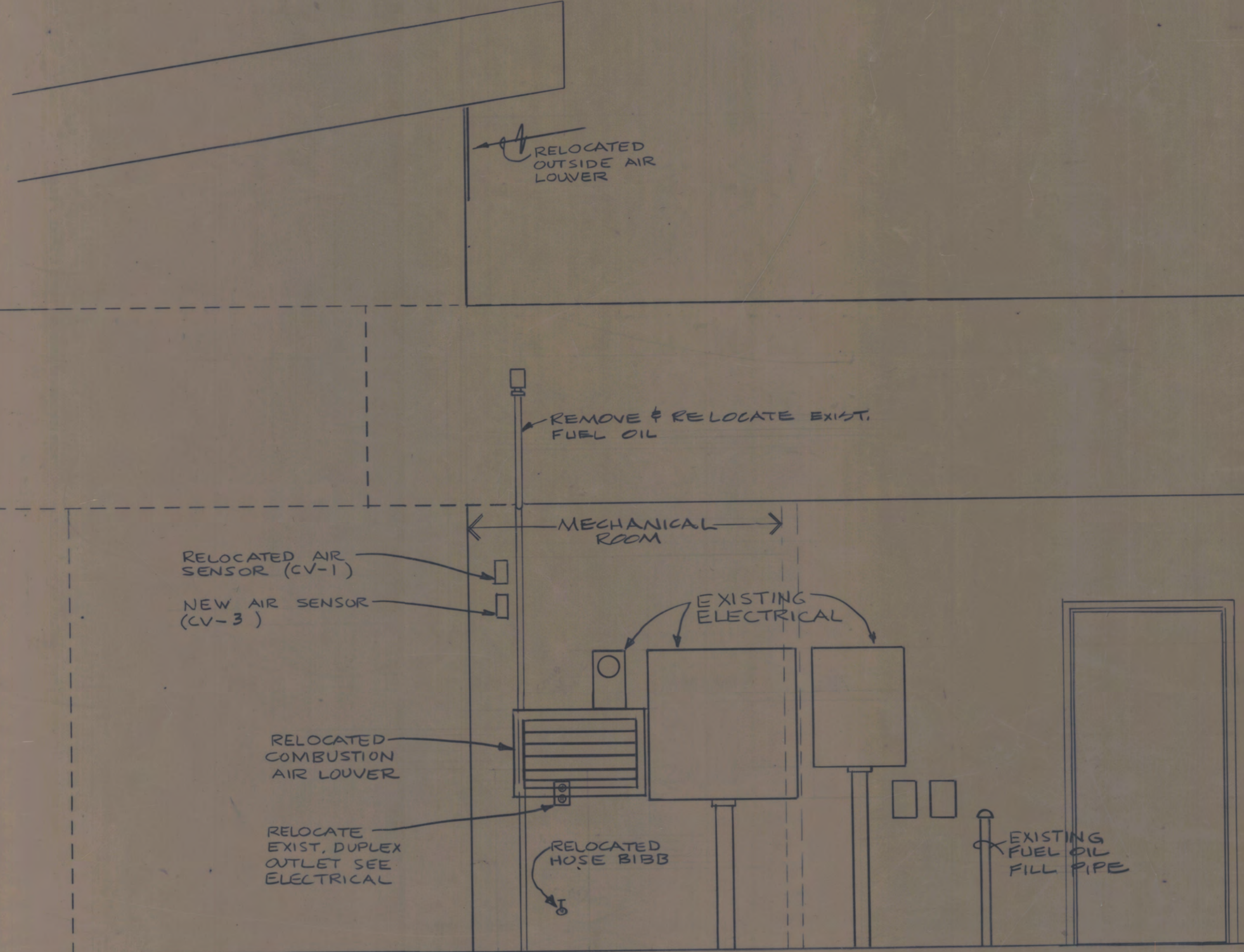
1 EXISTING MECH. RM NORTH ELEVATION M-4 1/2" = 1'-0"
