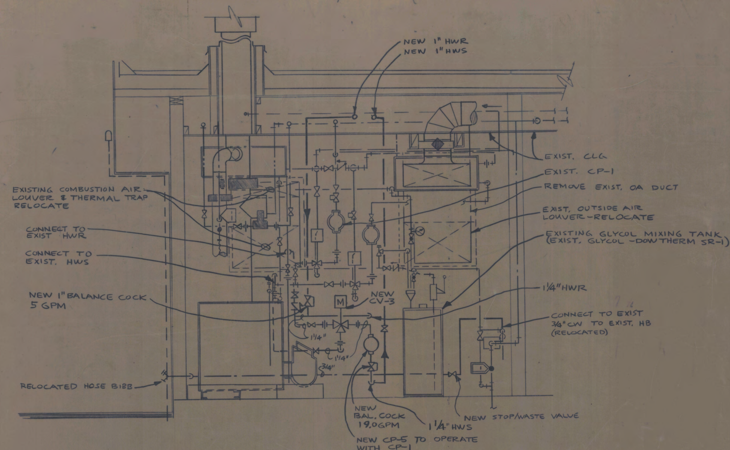
1 EXISTING MECH. RM NORTH ELEVATION M-4 1/2" = 1'-0"
