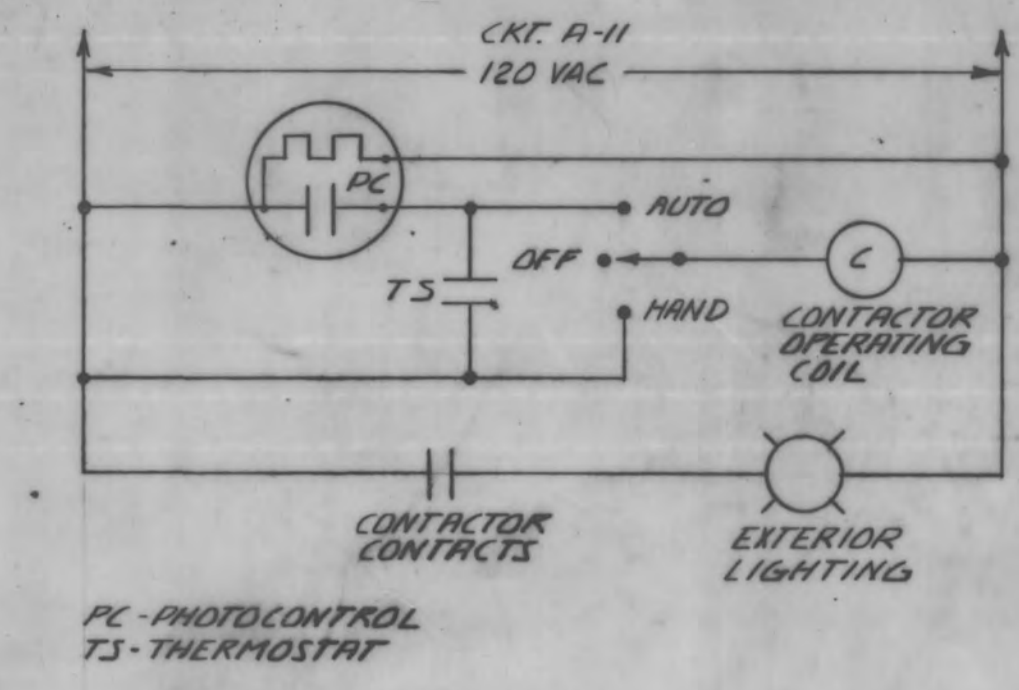
1 E-2 OUTSIDE LIGHTING CONTROL DIAGRAM
