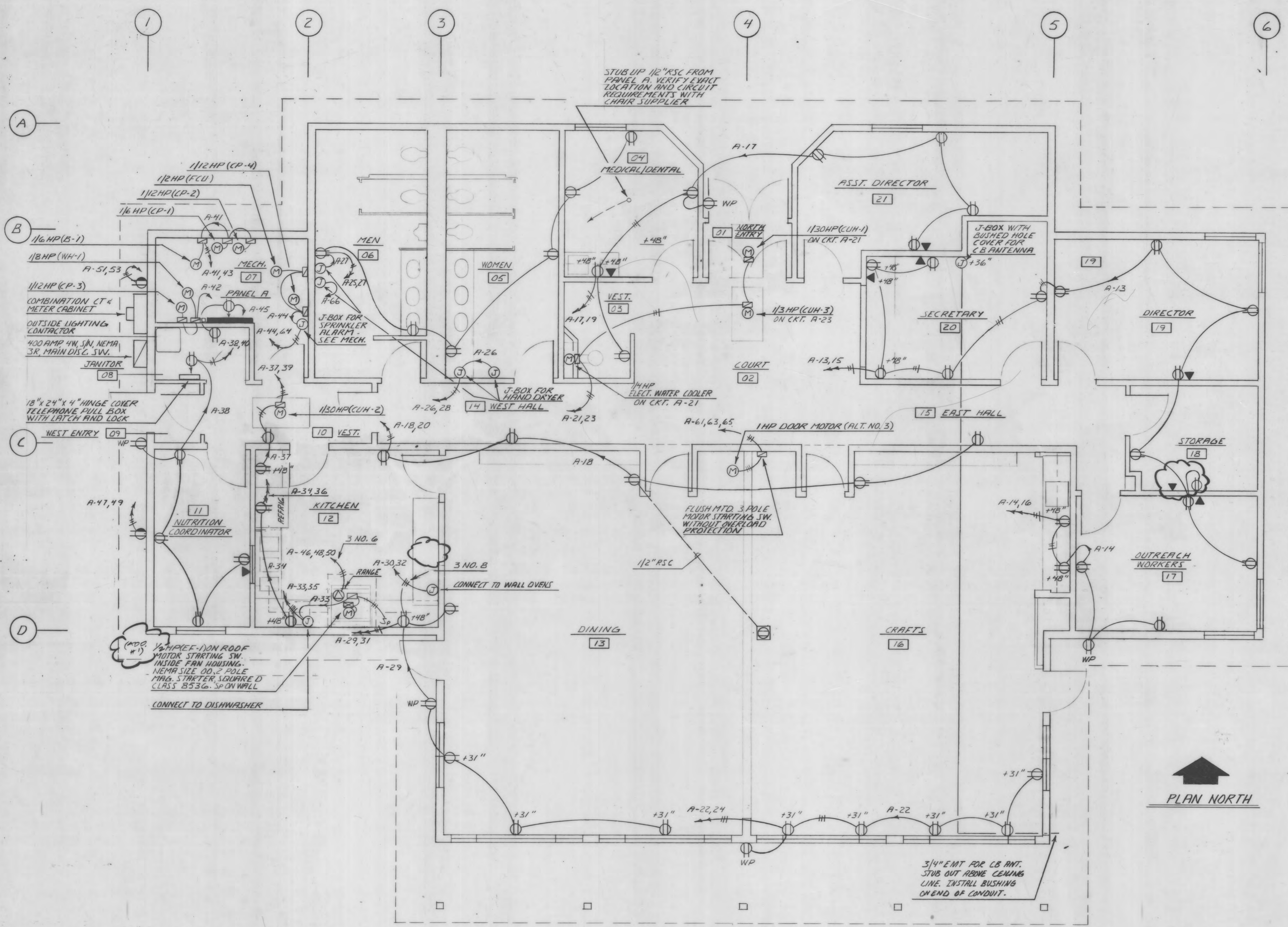
POWER PLAN SCALE 1/4" = 1'-0"
