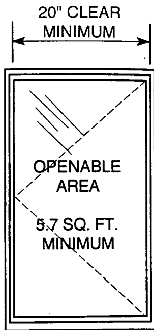
MINIMUM SIZE WINDOW FOR 20" CLEAR WIDTH
