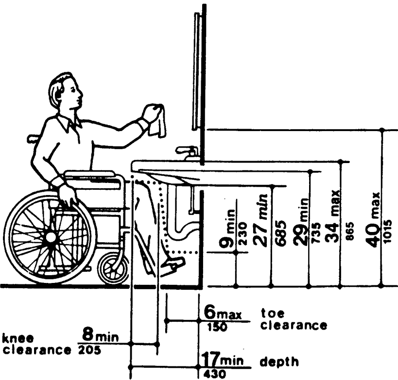
Fig. 31 Lavatory Clearances
